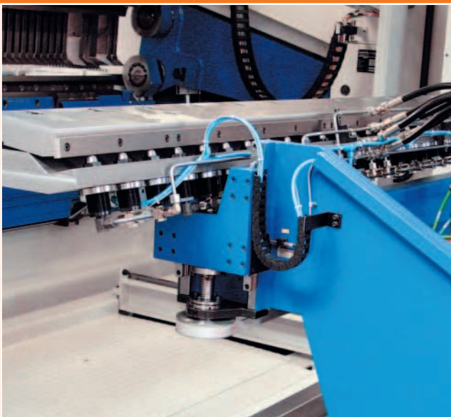
Option DF is a patented hydraulic folding system for lengths up to 3 m. It can either be integrated into the back of the B12 or operated by robot as an independent station.
