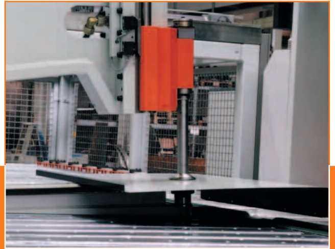
Option LKNU is used for workpieces with negative (downward-facing) folds. The manipulator lifts the piece into the normal unloading position.
