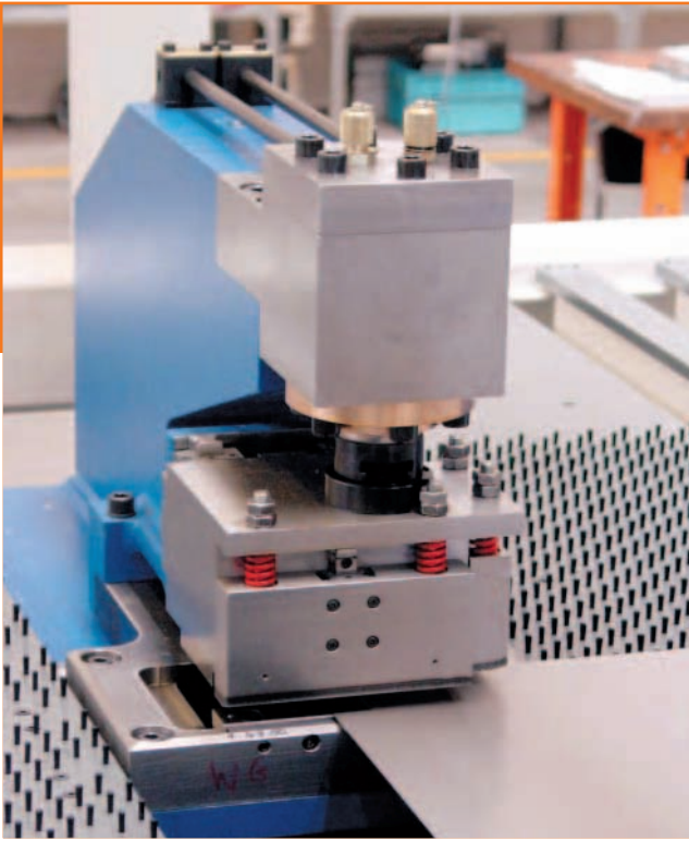
Integrated into the loading area: Option K4R. 4 CNC-adjustable notching units can perform multiple notching operations during the main bending process.
